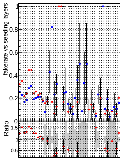
Fake rate vs. DQM V0001_R000000001 Global cmssw RECO Fake rate vs. DQM V0001_R000000001 Global mkFitNew RECO
