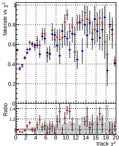
Fake rate vs. —●— DQM V0001_R000000001 Global cmssw RECO —●— DQM V0001_R000000001 Global mkFitNew RECO
