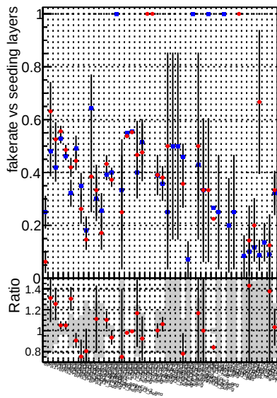
Fake rate vs. —●— DQM V0001_R000000001 Global cmssw RECO —●— DQM V0001_R000000001 Global mkFitNew RECO
