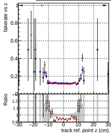
Legend: ■ DQM_V0001_R000000001_Global_cmssw_RECO ● DQM_V0001_R000000001_Global_mkFitNew_RECO
