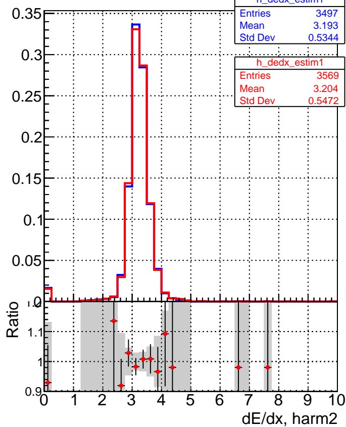
—■ DQM_V0001_R000000001_Global_cmssw_RECO —● DQM_V0001_R000000001_Global_mkFitNew_RECO
