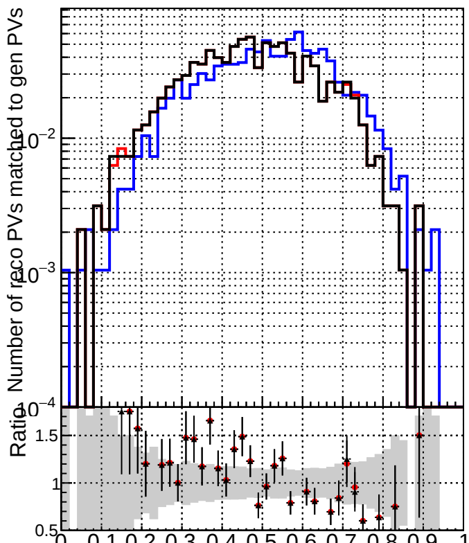
RecoPVAssoc2GenPVMatched_Purity
