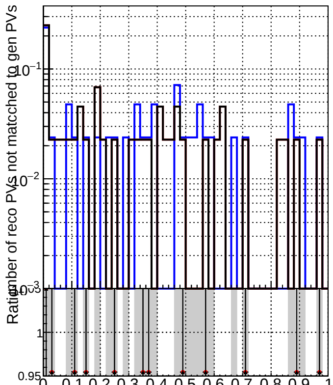
RecoPVAssoc2GenPVNotMatched_Purity
