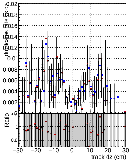
DOM V0001 R0000000001 Global cmssw RECO DOM V0001 R0000000001 Global mktFitOriginal RECO DOM V0001 R0000000001 Global mktFitNew RECO
