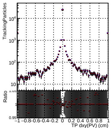
N of sim DQM_V0001_R000000001_Global_cmssw_RECO DQM_V0001_R000000001_Global_mkFitOriginal_RECO DQM_V0001_R000000001_Global_mkFitNew_RECO
