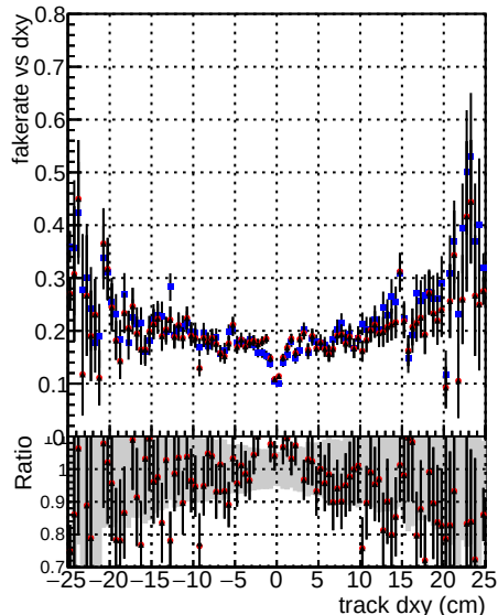
DOM V0001 R0000000001 Global fit New RECO DOM V0001 R0000000001 Global fit Original RECO
