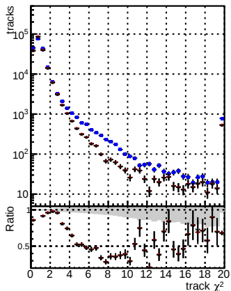
N of reco track vs. s DOM V0001 R0000000001 Global mkFitOriginal RECO DOM V0001 R0000000001 Global mkFitNew RECO DOM V0001 R0000000001 Global mkFitNew RECO
