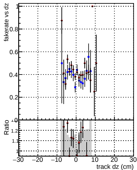
Fake rate vs dz Legend: DOM V0001 R0000000001 Global cmssw RECO DOM V0001 R0000000001 Global mkFitOriginal RECO DOM V0001 R0000000001 Global mkFitNew RECO
