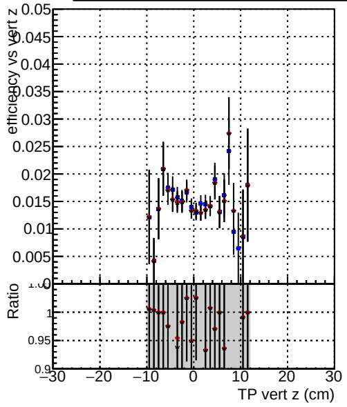
Efficiency vs. TP vert z (cm) —●— DQM_V0001_R0000000001_Global_cmssw_RECO —●— DQM_V0001_R0000000001_Global_mkFitOriginal_RECO —●— DQM_V0001_R0000000001_Global_mkFitNew_RECO
