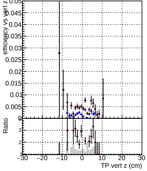
Efficiency vs. sim PV z —●— DQM_V0001_R000000001 Global_cmssw_RECO —●— DQM_V0001_R000000001 Global_mkFitOriginal_RECO —●— DQM_V0001_R000000001 Global_mkFitNew_RECO
