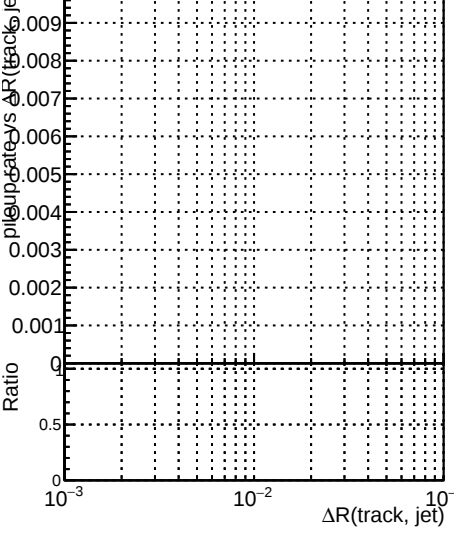
Pileup rate vs \Delta R (track, jet)
