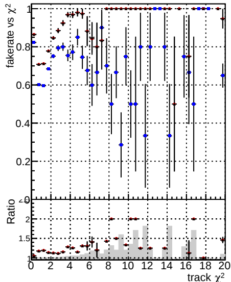
Fake rate vs. Legend DOM V0001 R0000000001 Global cmssw RECO Blue line with dots DOM V0001 R0000000001 Global cmssw RECO Red line with dots DOM V0001 R0000000001 Global mkFitOriginal RECO Gray shaded region DOM V0001 R0000000001 Global mkFitNew RECO
