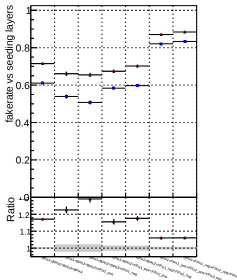
Fake rate vs. Legend DOM V0001 R0000000001 Global cmssw RECO Blue line with dots DOM V0001 R0000000001 Global cmssw RECO Red line with dots DOM V0001 R0000000001 Global mkFitOriginal RECO Gray shaded region DOM V0001 R0000000001 Global mkFitNew RECO
