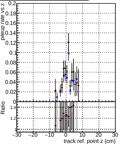
Legend for all plots: —•— DQM_V0001_R000000001 Global cmssw RECO —•— DQM_V0001_R000000001 Global mkFitOriginal RECO —•— DQM_V0001_R000000001 Global mkFitNew RECO
