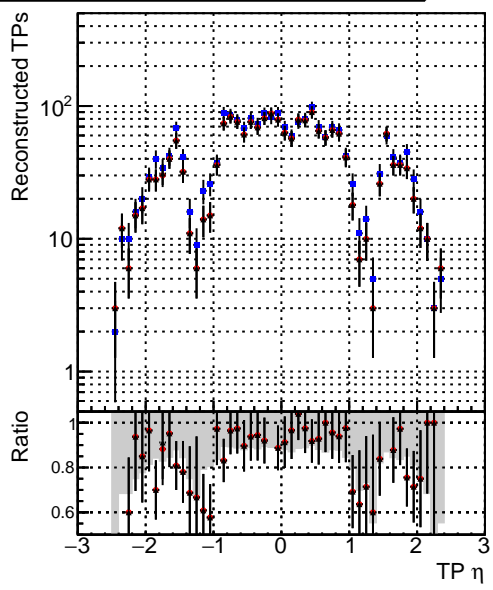
N of simulated tracks vs \eta Legend: DQM_V0001_R000000001_Global_cmssw_RECO DQM_V0001_R000000001_Global_mkFitOriginal_RECO DQM_V0001_R000000001_Global_mkFitNew_RECO
