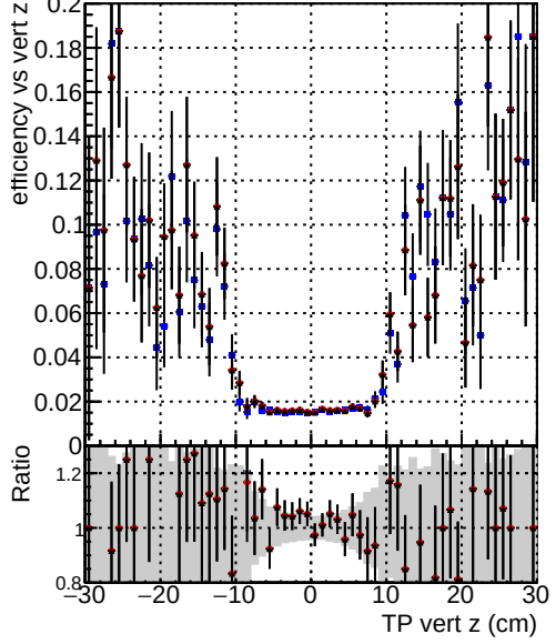
Efficiency vs vert z Global_cmssw_RECO Global_mkFitOriginal_RECO Global_mkFitNew_RECO
