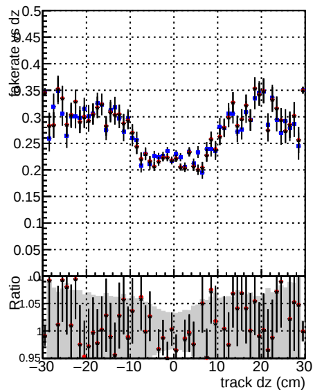
DOM V0001 R0000000001 Global cmssw RECO DOM V0001 R0000000001 Global mktFitOriginal RECO
