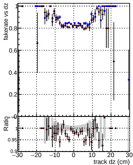
DOM V0001 R0000000001 Global fit cms sw RECO DOM V0001 R0000000001 Global fit mkFitOriginal RECO DOM V0001 R0000000001 Global fit mkFitNew RECO
