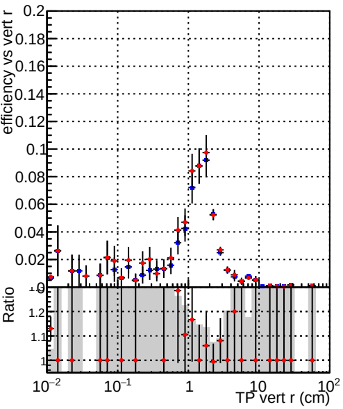
Efficiency vs vertpos Legend: DQM_TT_original (blue squares), DQM_TT_newscore (red stars)
