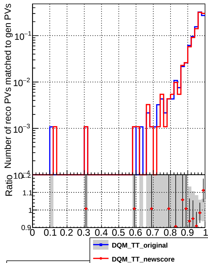
RecoPVAssoc2GenPVmatched_missing
