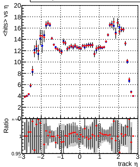
mean hits — DQM_TT_original — DQM_TT_newscore
