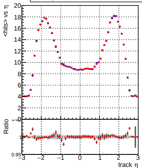
mean hit — DQM_TT_original — DQM_TT_newscore
