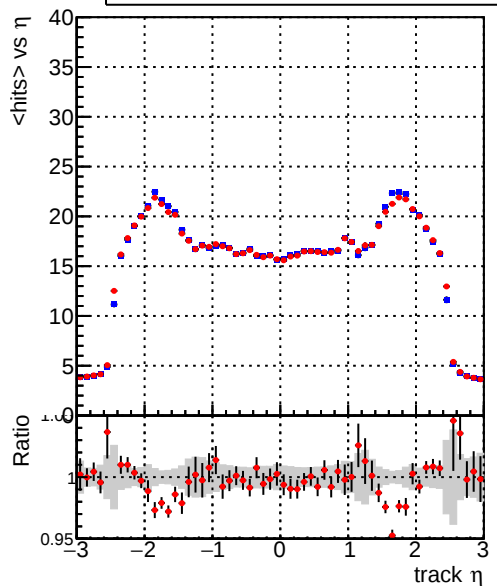
mean hits DQM_TT_original DQM_TT_newscore
