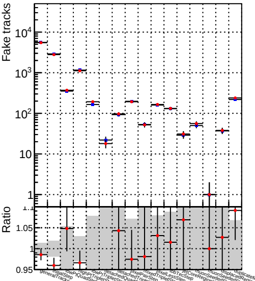
Number —●— DQM_TT_newscore
