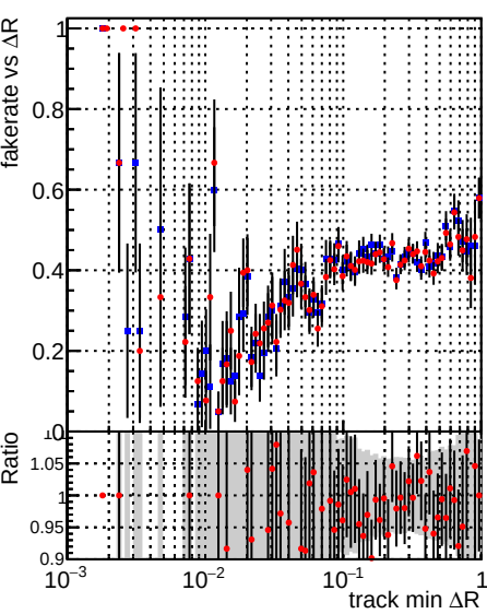
Legend: DQM_TT_original (blue), DQM_TT_newscore (red)
