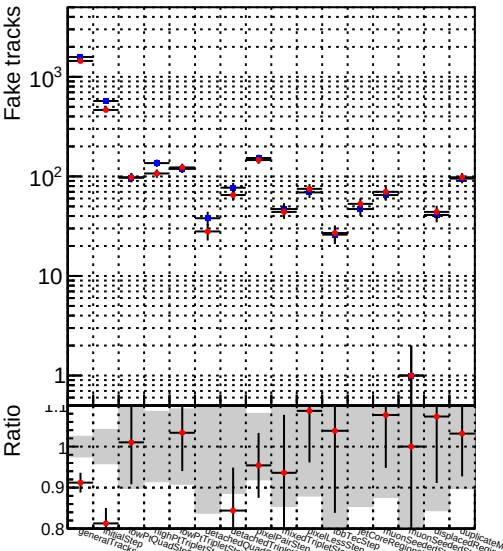
Number —●— DQM_TT_newscore
