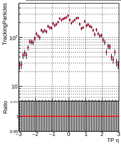
N of simulated tracks vs \eta Legend: DQM_TT_original (blue line), DQM_TT_newscore (red line)
