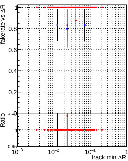
Legend: DQM_TT_original DQM_TT_newscore
