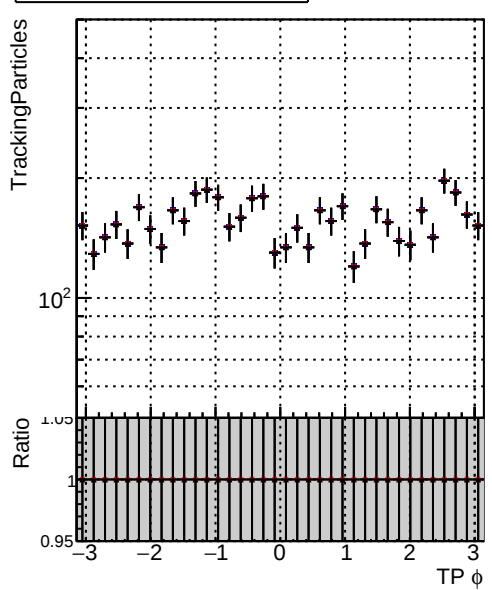
N of simulated tracks vs phi-TP
