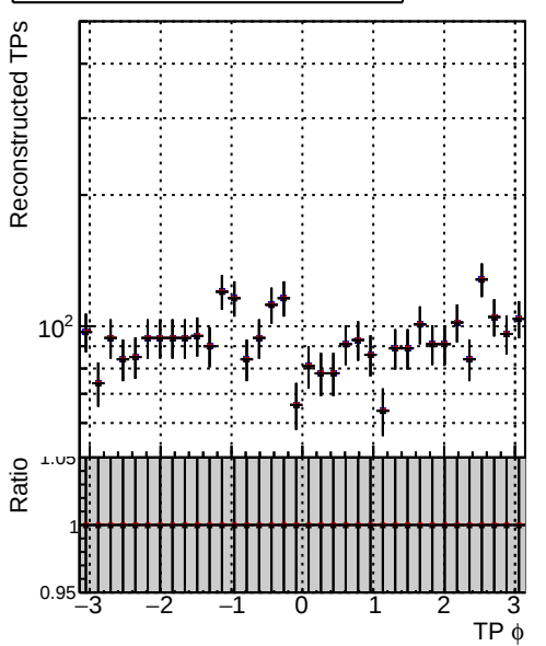
N of associated tracks (simToReco) vs phi-TP
