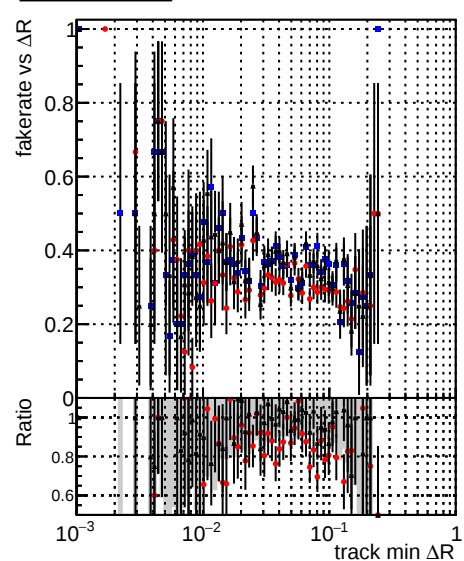
Fake rate vs \Delta R (track, jet) Legend: \Delta R (black) \Delta R (blue) \Delta R (red) \Delta R (black) \Delta R (blue) \Delta R (red)
