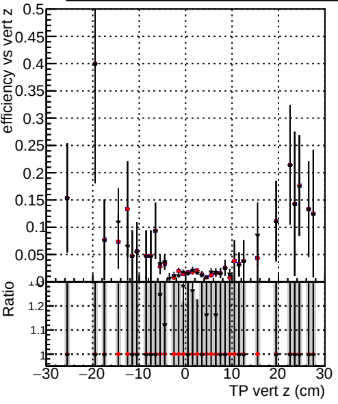
Efficiency vs TP vert z Legend: DQM_TT_original_time DQM_TT_original_time2 DQM_TT_modified_time2
