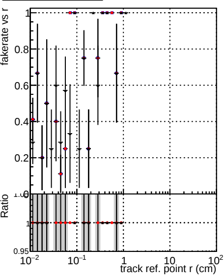
Fake rate vs v Legend: DQM TT original time DQM TT original time2 DQM TT modified time2
