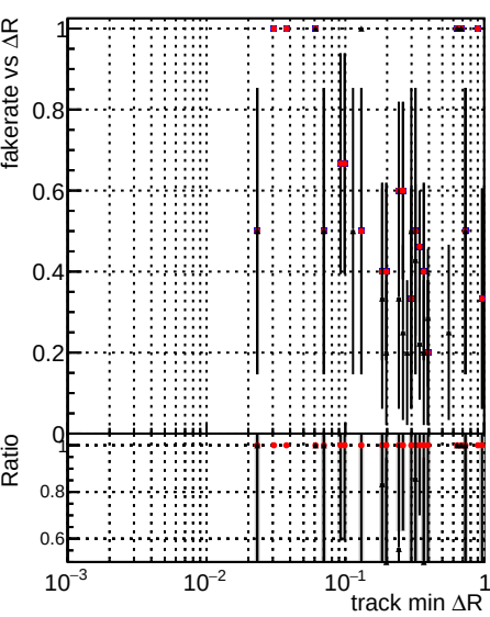
Fake rate vs \Delta R(\text{track, jet}) Legend: DQM TT original time DQM TT original time2 DQM TT modified time2
