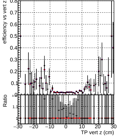
Efficiency vs. TP vert z (cm) — DQM_TT_original_time — DQM_TT_original_time2 — DQM_TT_modified_time2
