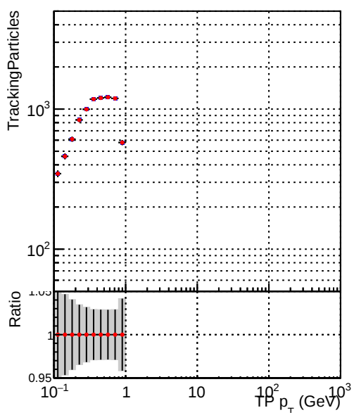
Legend: \blacksquare DQM_TT_original_time \bullet DQM_TT_modified_time
