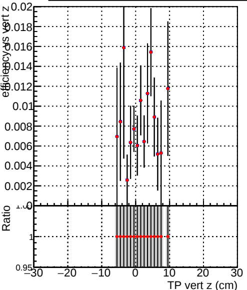
Efficiency vs TP vert z (cm) Legend: DQM_TT_original_time (grey bars) DQM_TT_modified_time (red dots)
