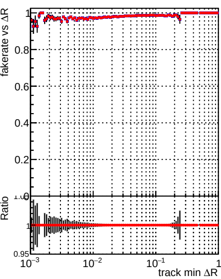
Fake rate vs \Delta R (track, jet) DQM_TT_original_time DQM_TT_modified_time
