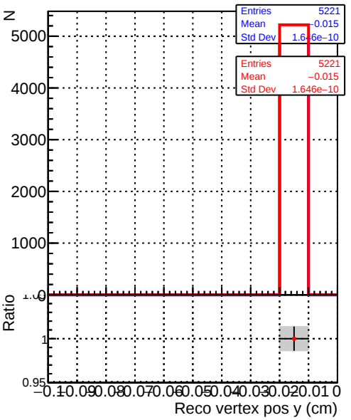
ReconstructedAllAssoc2Gen_Y
