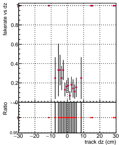
Fake rate vs dz —•— DQM_TT_original_time —•— DQM_TT_modified_time
