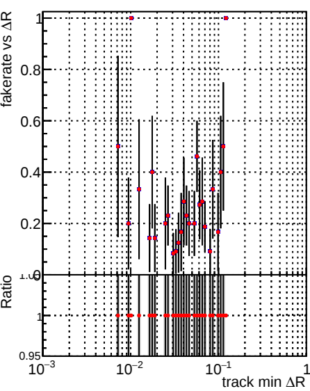
Fake rate vs \Delta R(\text{track, jet}) Legend: \Delta R(\text{track, jet}) (grey line with error bars) \Delta R(\text{track, jet}) (red line with error bars)
