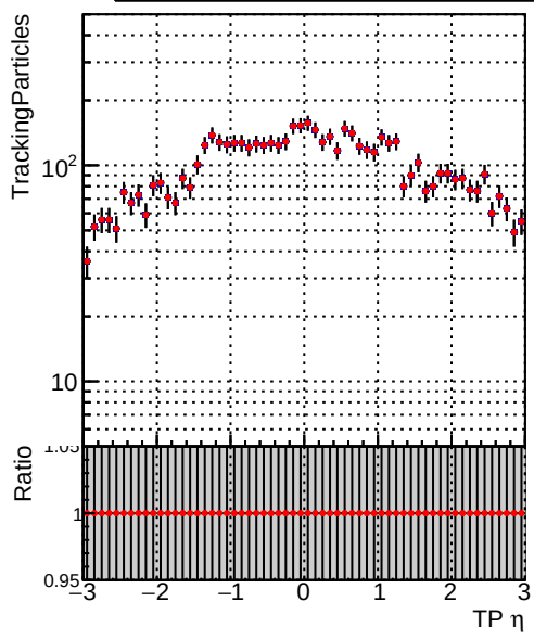
N of simulated tracks vs TP \eta Legend: DQM_TT_original_time (blue line with dots), DQM_TT_modified_time (red line with dots)
