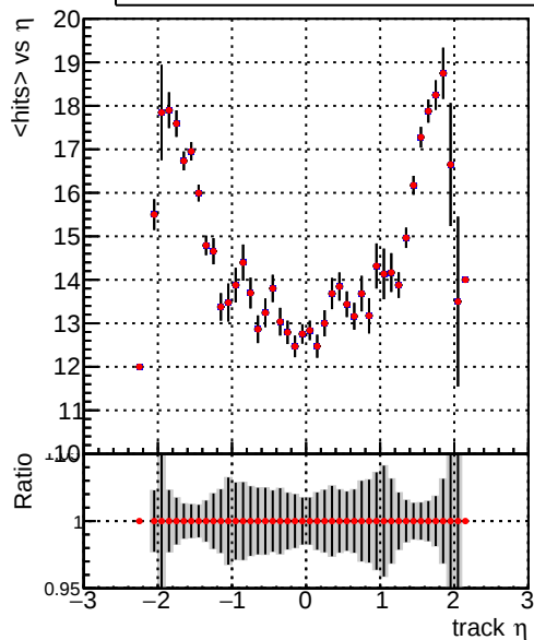
mean hits vs \eta — DQM_TT_original_time — DQM_TT_modified_time
