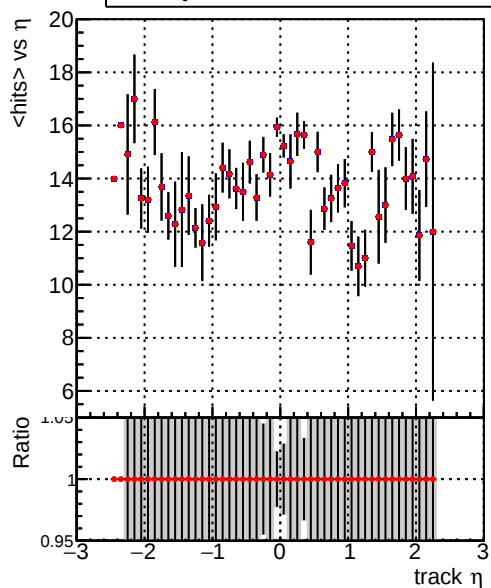
mean hits — DQM_TT_original_time — DQM_TT_modified_time
