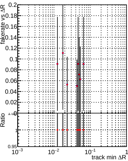
Fake rate vs ΔR(track, jet) DQM_TT_original_time DQM_TT_modified_time
