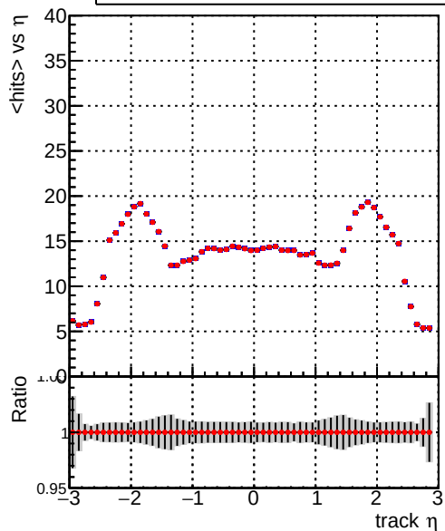
mean hits — DQM_TT_original_time — DQM_TT_modified_time
