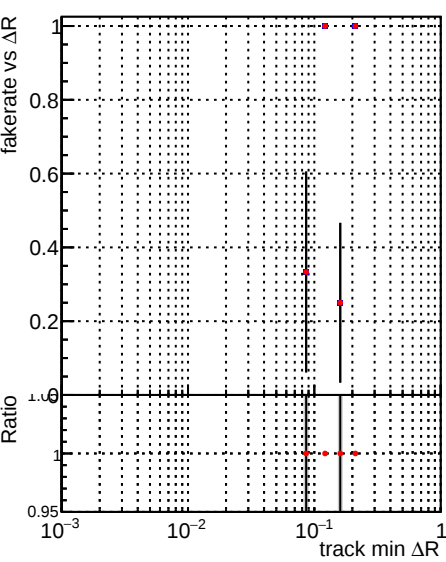
Fake rate vs \Delta R(\text{track, jet}) Legend: — DQM_TT_original_time — DQM_TT_modified_time
