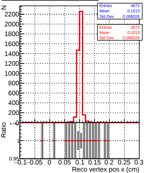
ReconstructedAllAssoc2Gen_X
