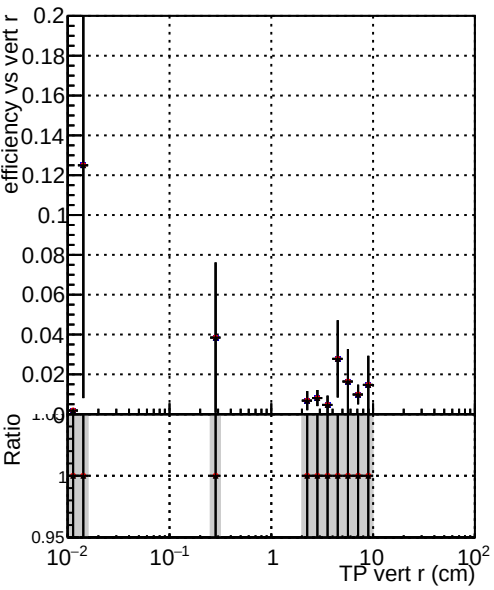
Efficiency vs TP vert r (cm) DQM_TT_original_time DQM_TT_newscoreonlyINIT_time DQM_TT_modified_time
