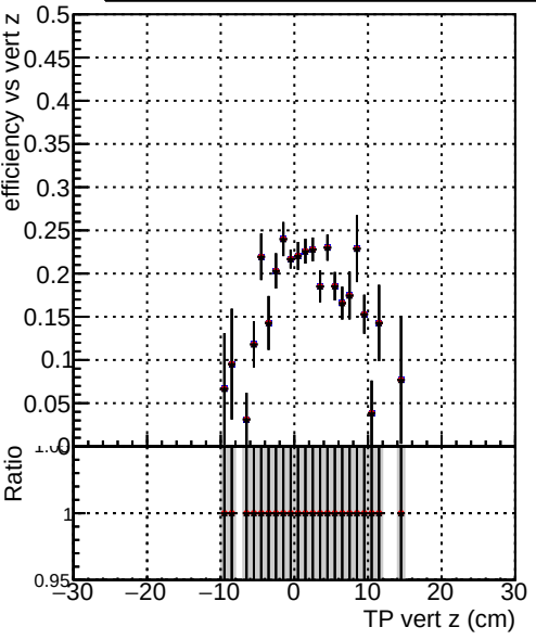
Efficiency vs vertpos DQM_TT_original_time DQM_TT_newscoreonlyINIT_time DQM_TT_modified_time
